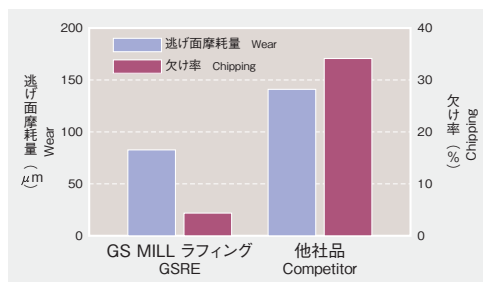
SKD11 (210HB) 溝加工の性能 Performance comparison of groove milling in SKD11(210HB)
