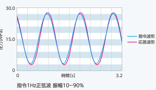
圧力正弦波応答
